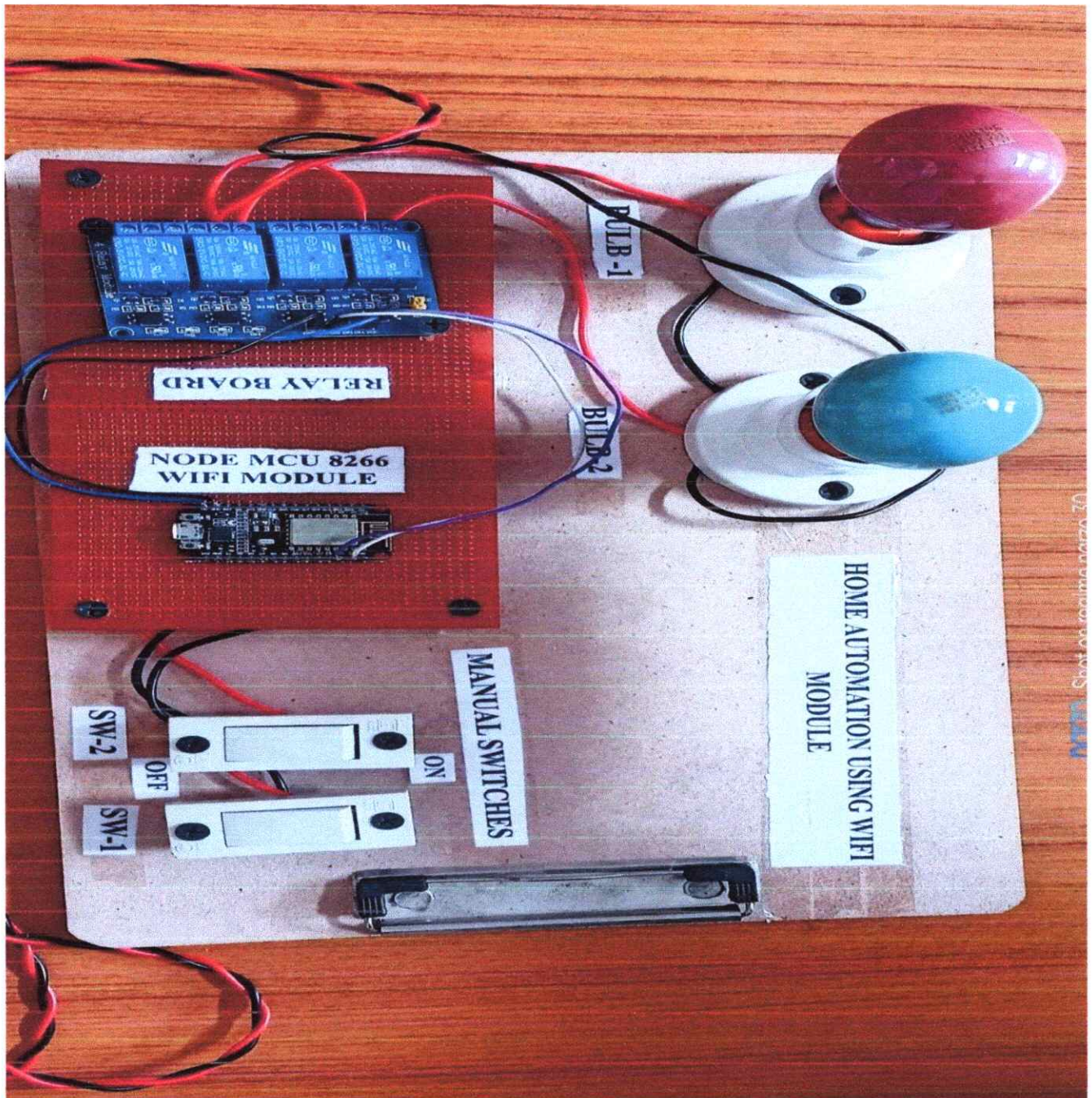
DESIGN HOME AUTOMATION USING WIFI MODULE
