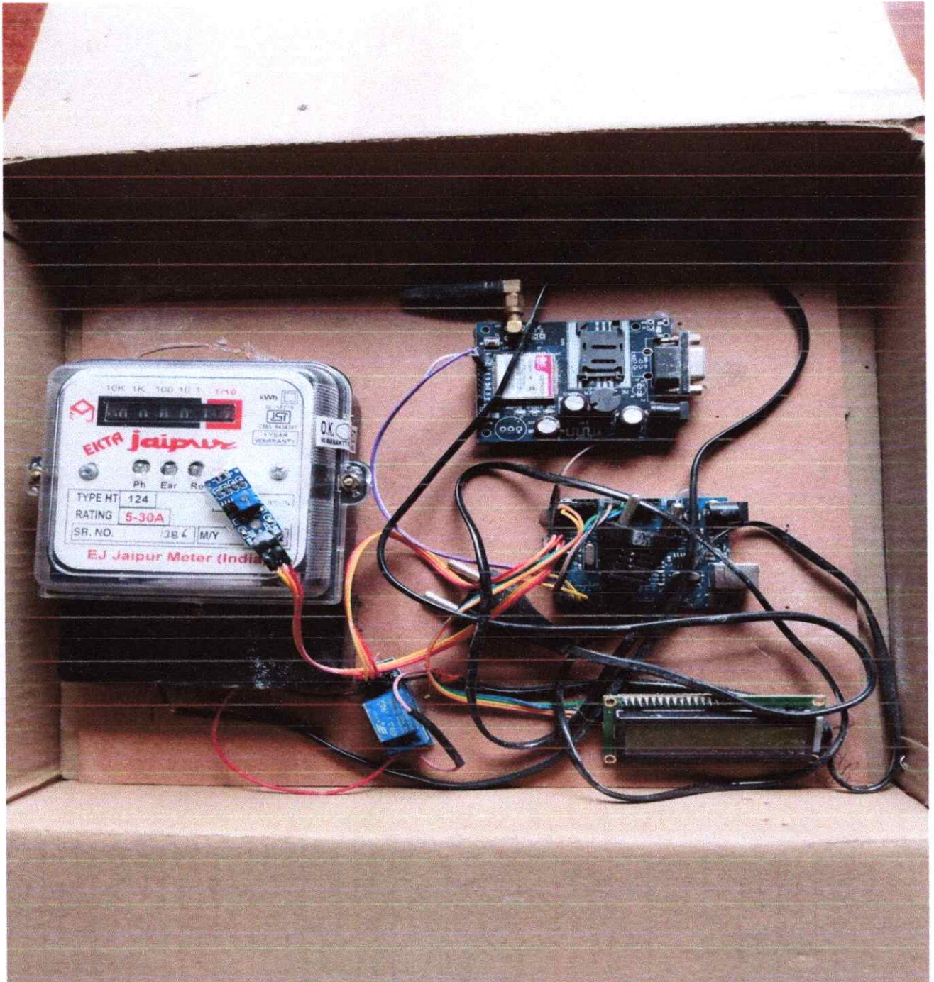
SMART ENERGY METER SYSTEM USING AURDIN AND GSM MODULE
