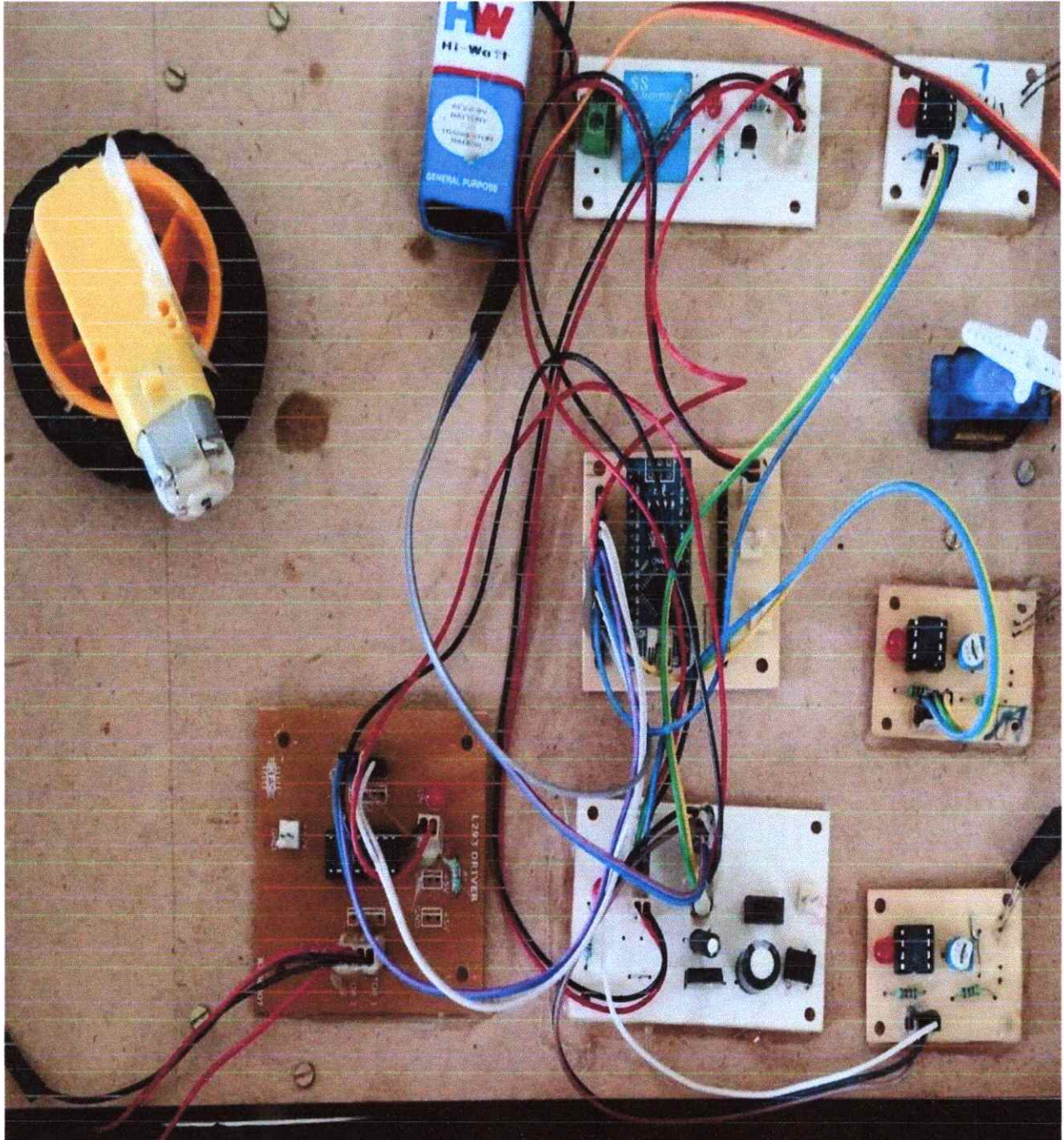
DESIGN OF FIRE FIGHTING ROBOT
