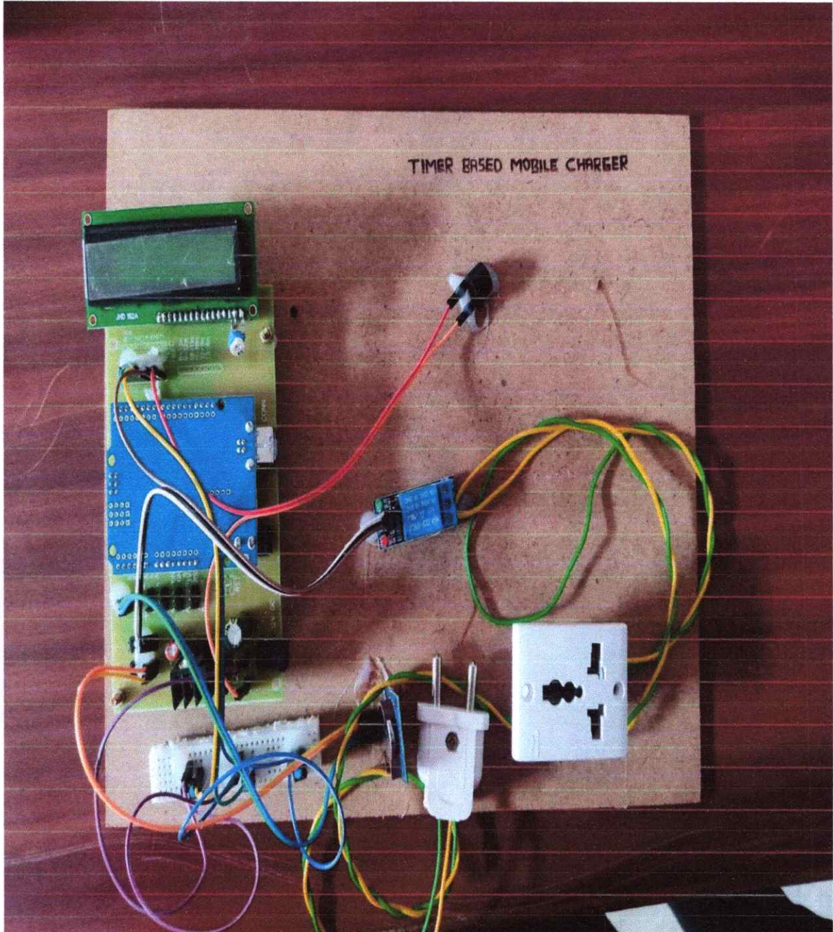
TIMER BASED MOBILE CHARGER
