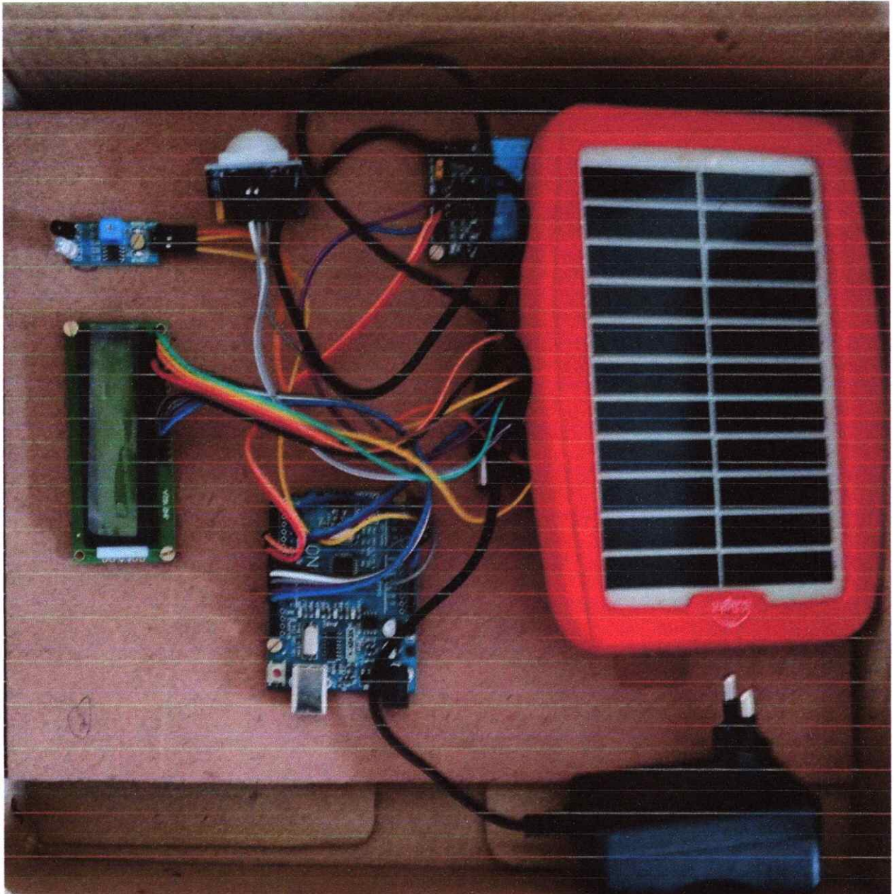
LIGHTING CONTROL SYSTEM IN RAILWAY STATION WITH SOLAR PANEL
