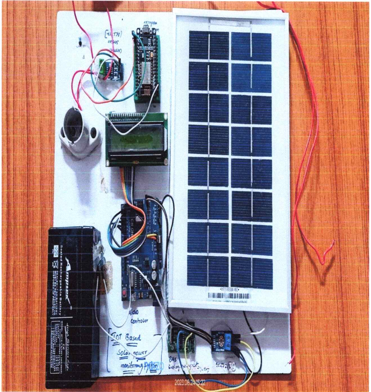
DESIGN IOT BASED SOLAR POWER MONITORING SYSTEM
