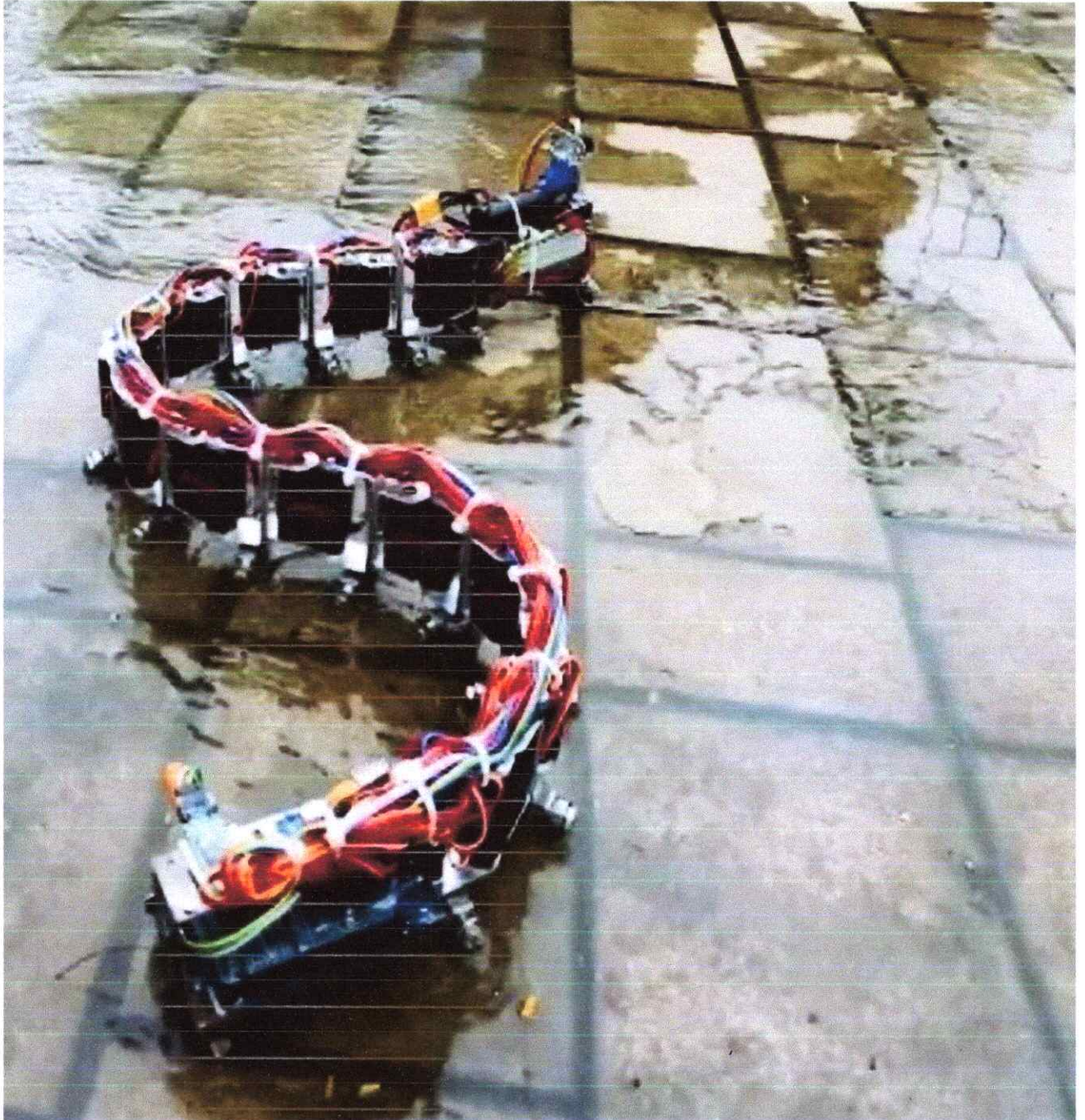
ARDUINO BASED SNAKE ROBOT CONTROLLED USING ANDROID APPLICATION
