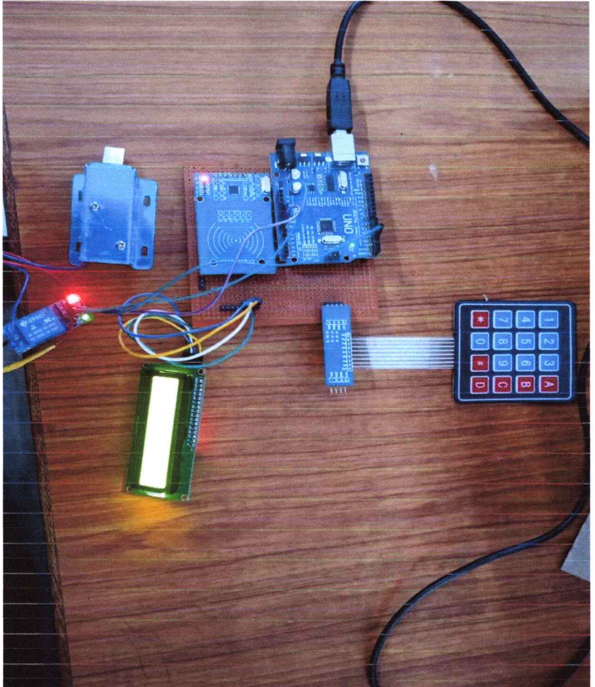
DESIGN & IMPLEMENTATION OF RFID & KEYPAD BASED LOCK SYSTEM
