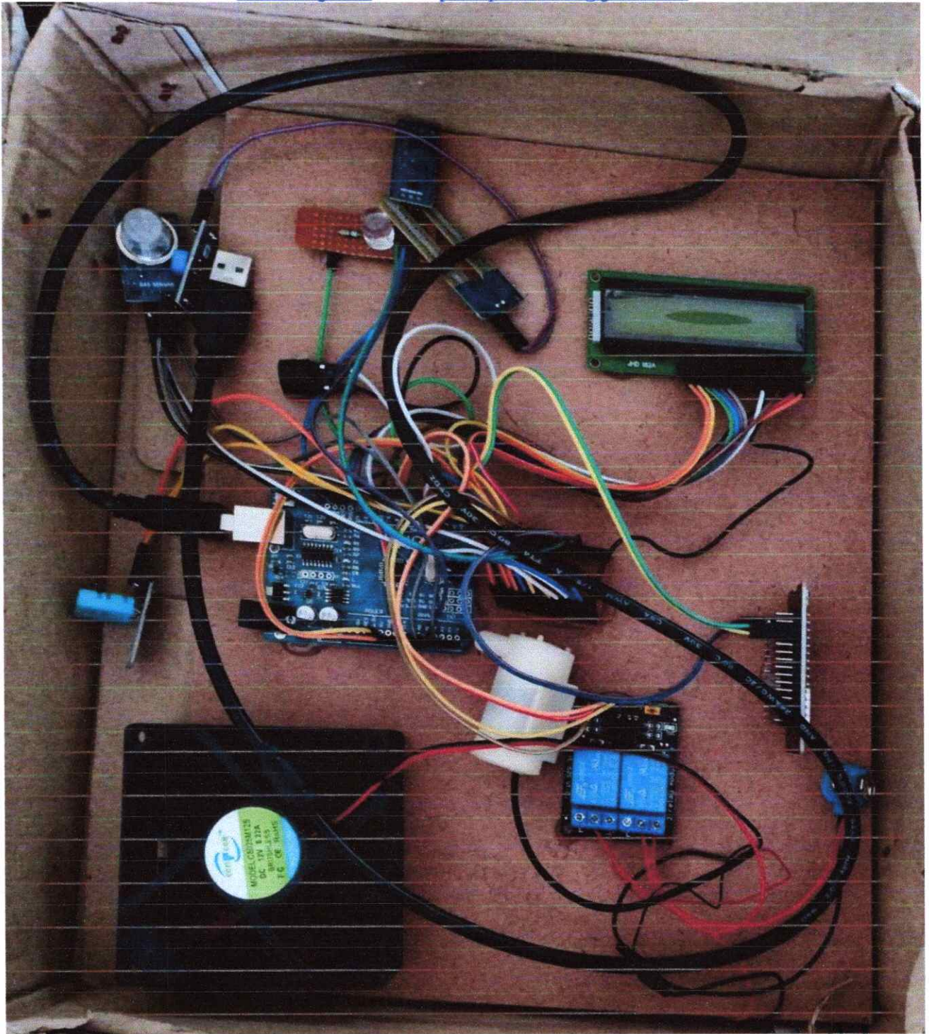
ENVIRONMENTAL MONITORING USING ARDUINO & IOT WITH ALERTING SYSTEM
