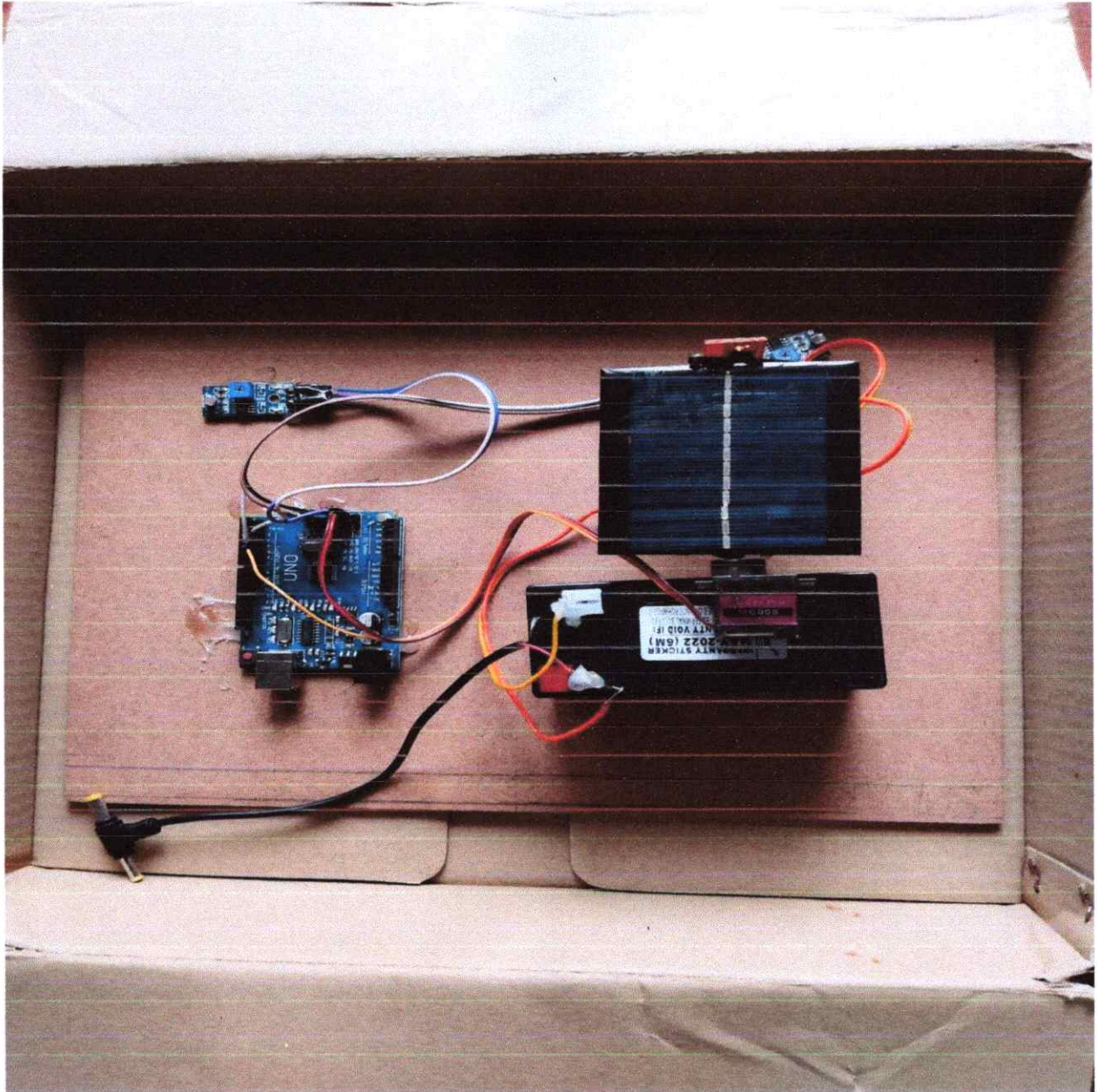
DESIGN SUN TRACKING SYSTEM FOR SOLAR GENERATION
